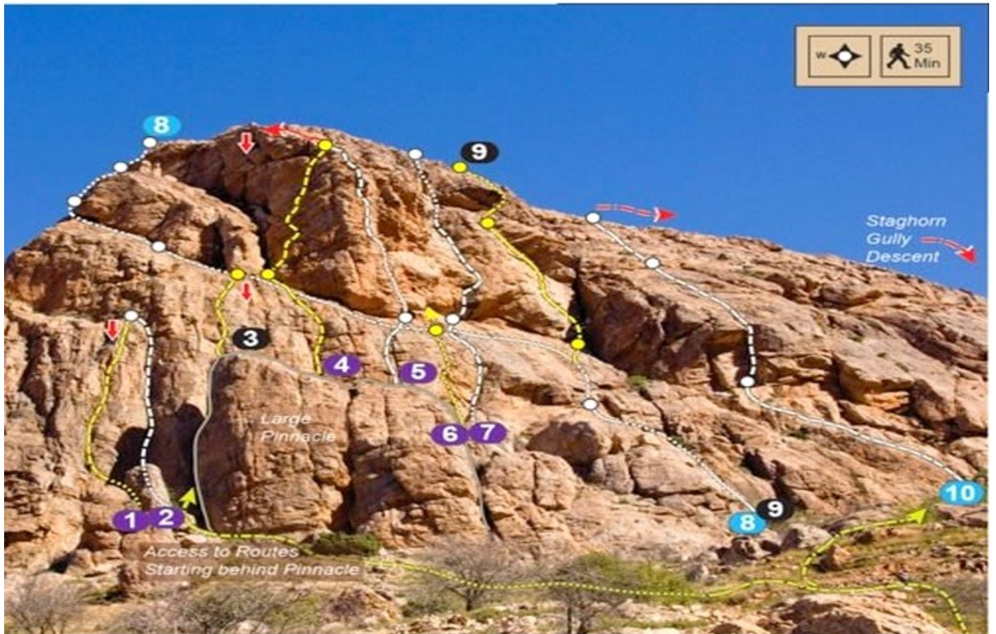
Morocco Rock - Jebel el Kest and Taskra North Overview Map (Géoparc Jbel Bani)
